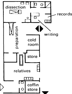
4 Mortuary, Municipal Hospital, Verbert (444 beds) Architects: Krüger, Krüger, Rieger
